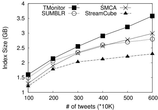
Fig. 10. Memory Usage
