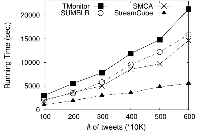
Fig. 9. Scalability
