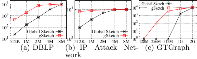
Figure 8: Number of Effective Queries for Edge Queries Q_e w.r.t. Memory Size (Bytes) (Zipf Skewness \alpha = 1.5 )
