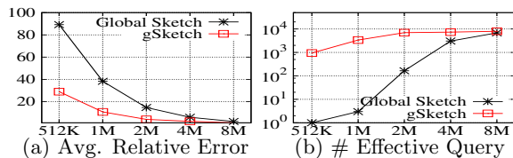
Figure 9: Query Estimation Accuracy of Graph Queries Q_g w.r.t. Memory Size (Bytes) in DBLP Data Set ( \alpha = 1.5 )
