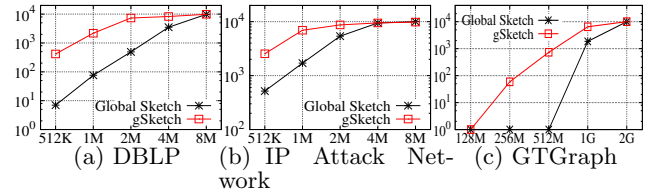
Figure 5: Number of Effective Queries for Edge Queries Q_e w.r.t. Memory Size (Bytes)
