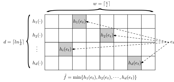
Figure 1: A CountMin Sketch
