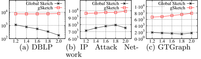
Figure 11: Number of Effective Queries for Edge Queries Q_e w.r.t. Zipf Sampling Skewness \alpha
